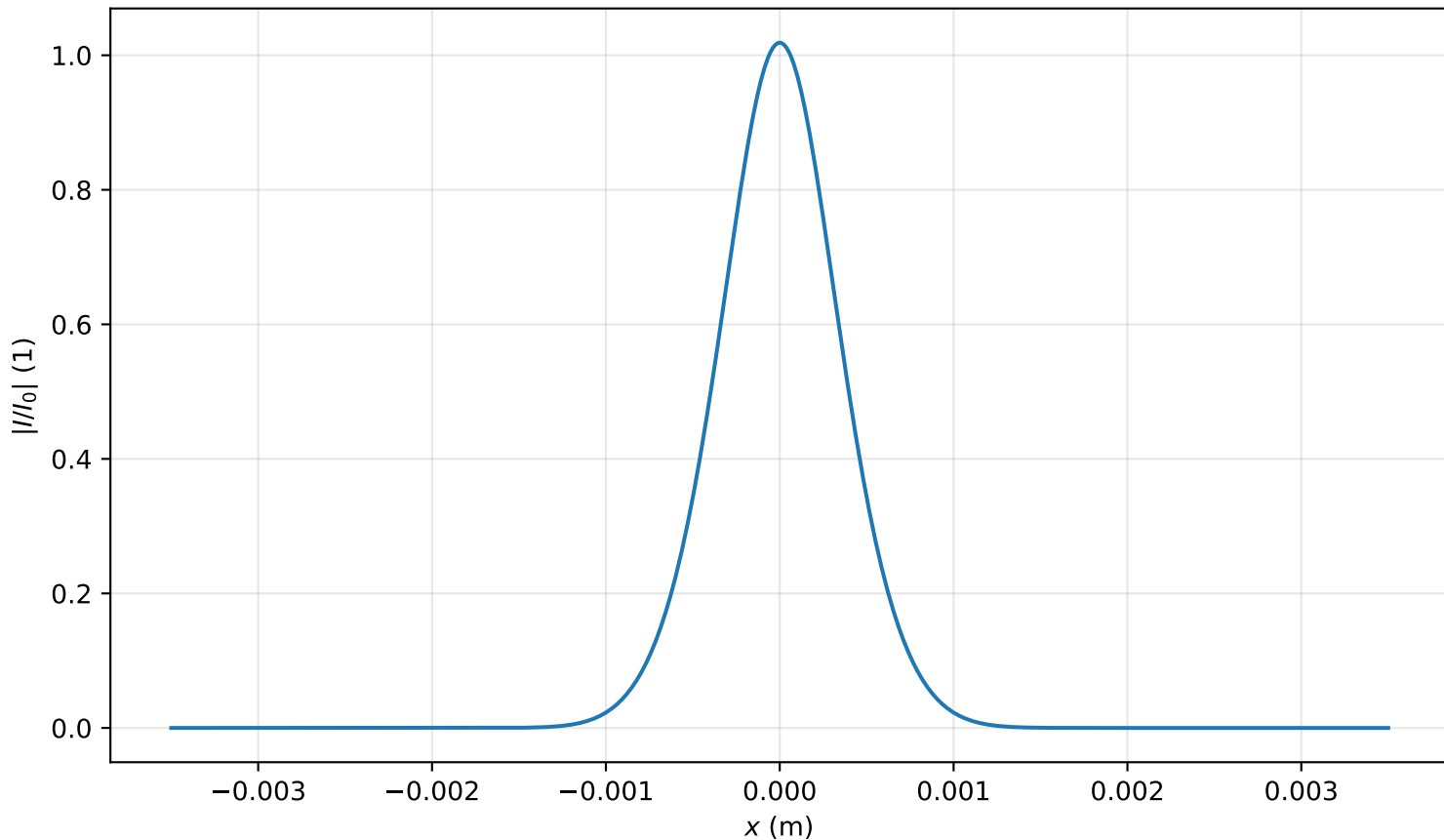
Intensity profile I(x, y = 0, z = 0.716m)/I_0 , P_{in}=0.4P_{cr} , artificial time
